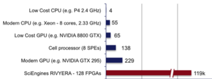
AES-128 decryption (million keys per second)
